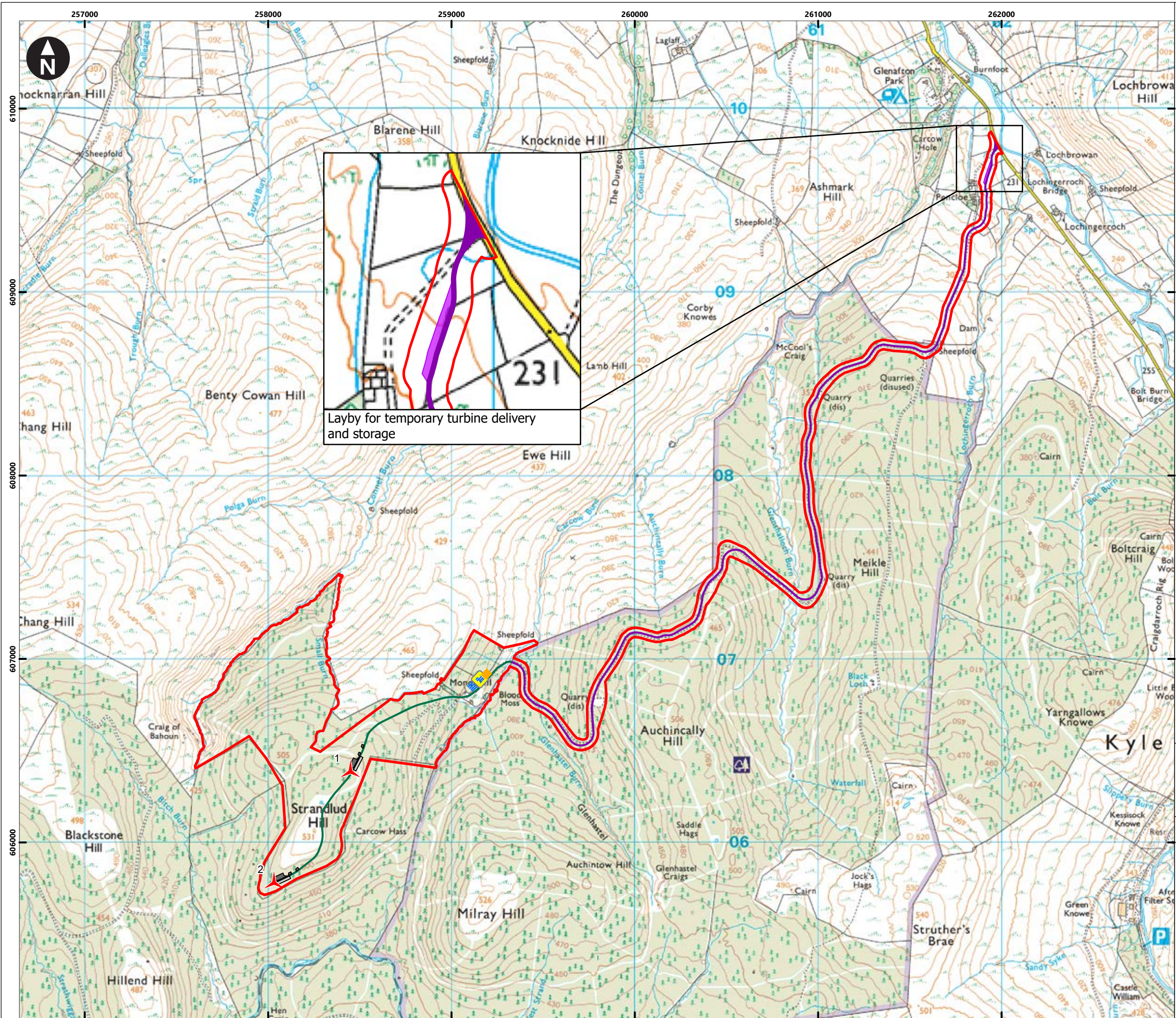
Figure 3.1 B Site Layout
