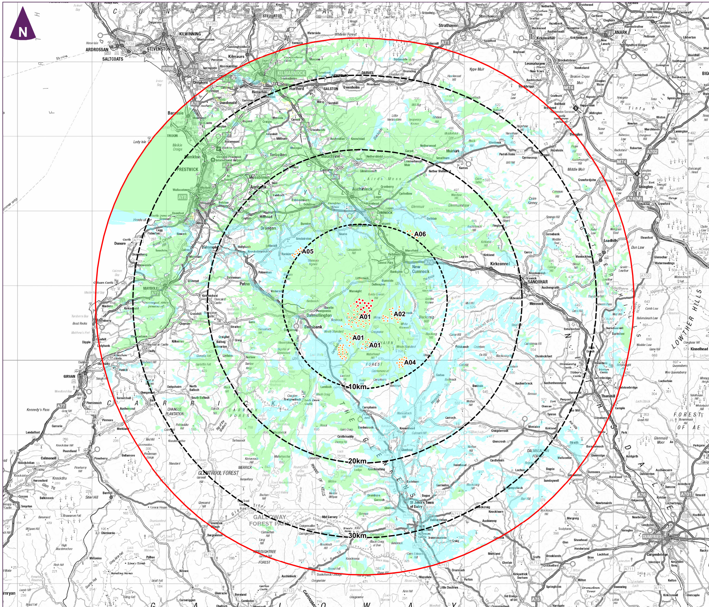
Figure 9.11a Cumulative ZTV 4a: Enoch and Application Wind Farms
