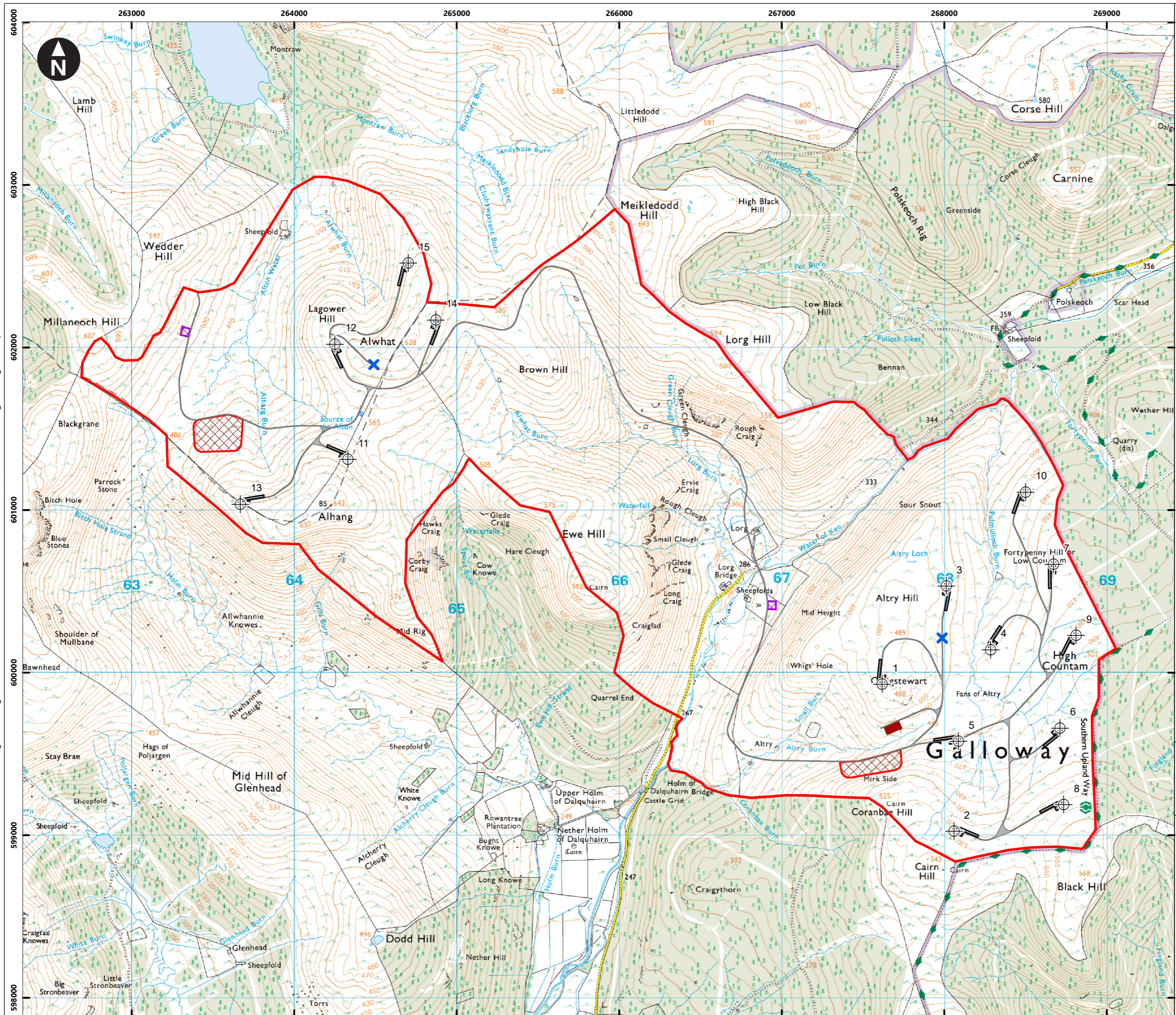
Figure 3.1a Site layout
